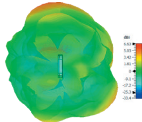
3D Plot Element A Side (5400MHz)
