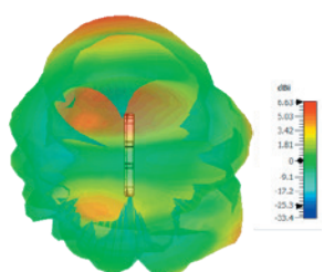
3D Plot Element A Top (5400MHz)
