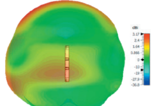
3D Plot Element A Top (2600MHz)
